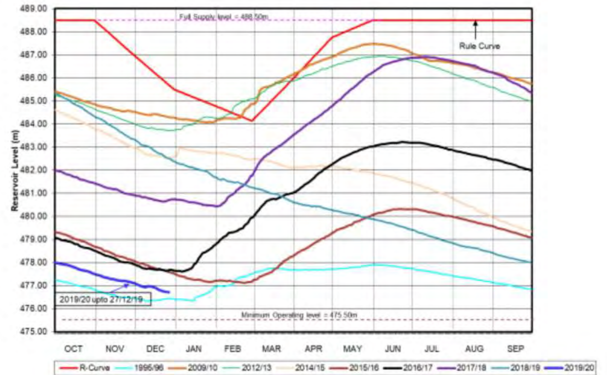
KARIBA RESERVOIR Comparison of Daily Reservoir Levels
